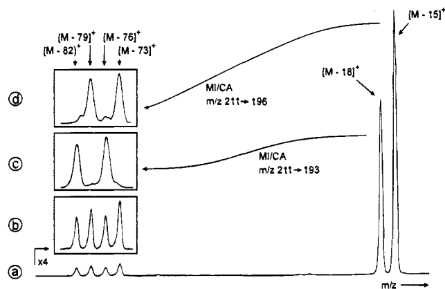
Figure 1. (a) Partial CA mass spectrum of 4a/Fe + (mass range: m/z 120–200; B2 scan). (b) Detail of the CA mass spectrum of 4a/Fe + magnified four times. (c) Detail of the MI/CA mass spectrum of 24a generated by unimolecular CH 3 • loss from 4a/Fe + (E2 scan). (d) Detail of the MI/CA mass spectrum of 24b generated by unimolecular CD 3 • loss from 4a/Fe + (E2 scan). The peak width in (a) differs from those in c and d due to the different scan methods.
